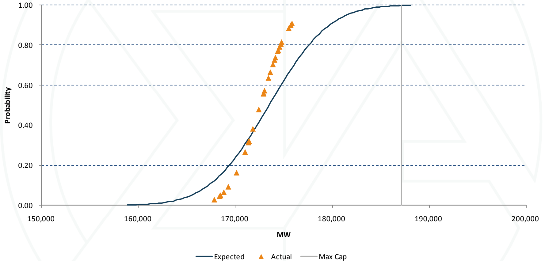
Distributions of Historical Performance vs EFORd Based Estimates: All Resources
