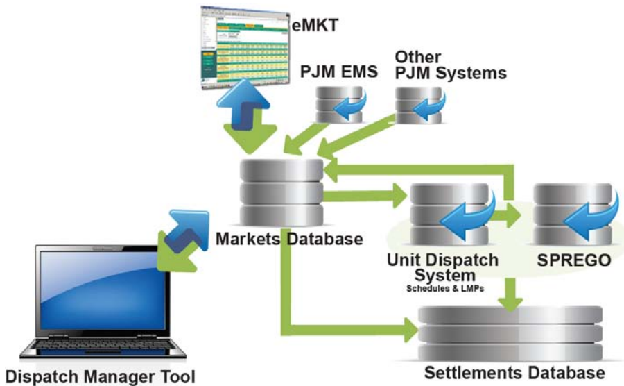
Exhibit 8: Synchronized Reserve and Regulation Subsystems
