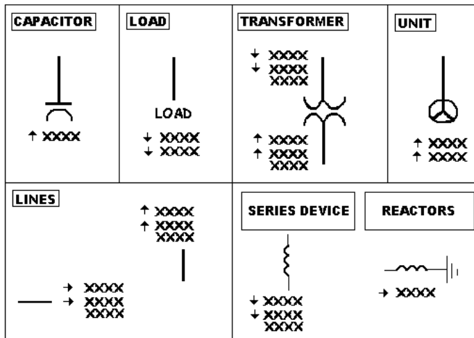
Exhibit 5 One-line diagram symbols
