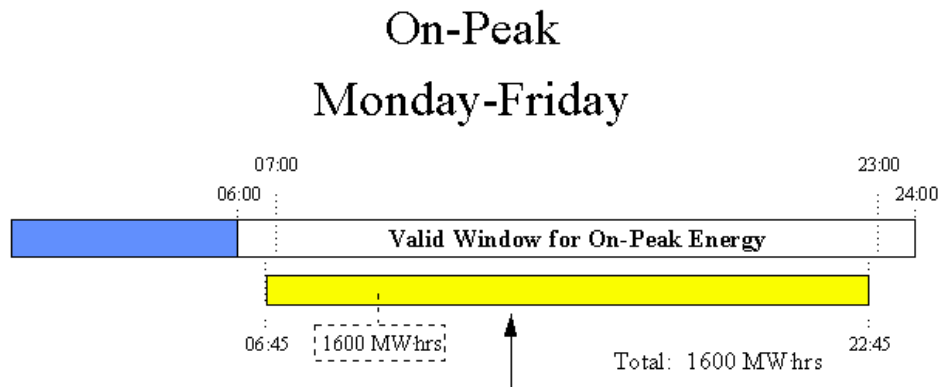
Example of Valid Energy Schedule using a 100MW Capacity On-Peak Transmission Service Reservation Over 16 Hour Period
