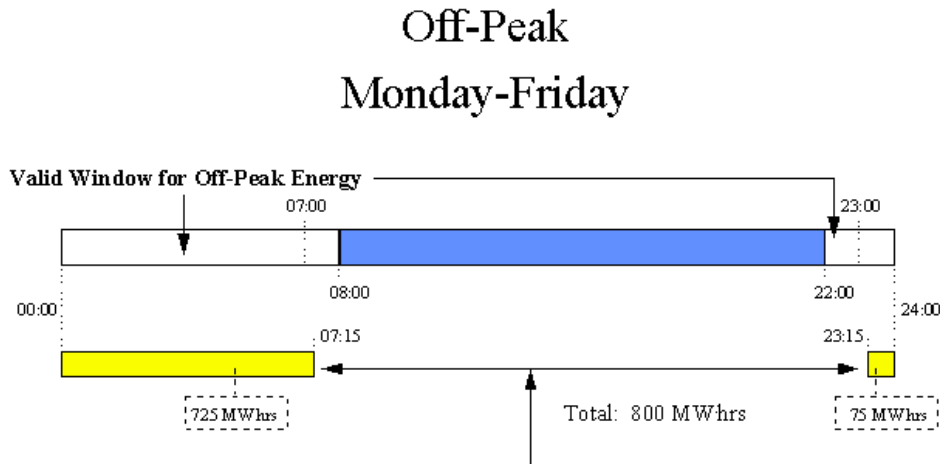
Example of Valid Energy Schedule using a 100MW Capacity Off-Peak Transmission Service Reservation
