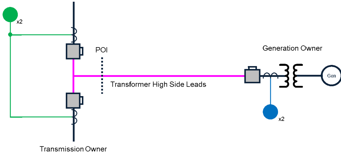
Figure 1. Acceptable Configuration
