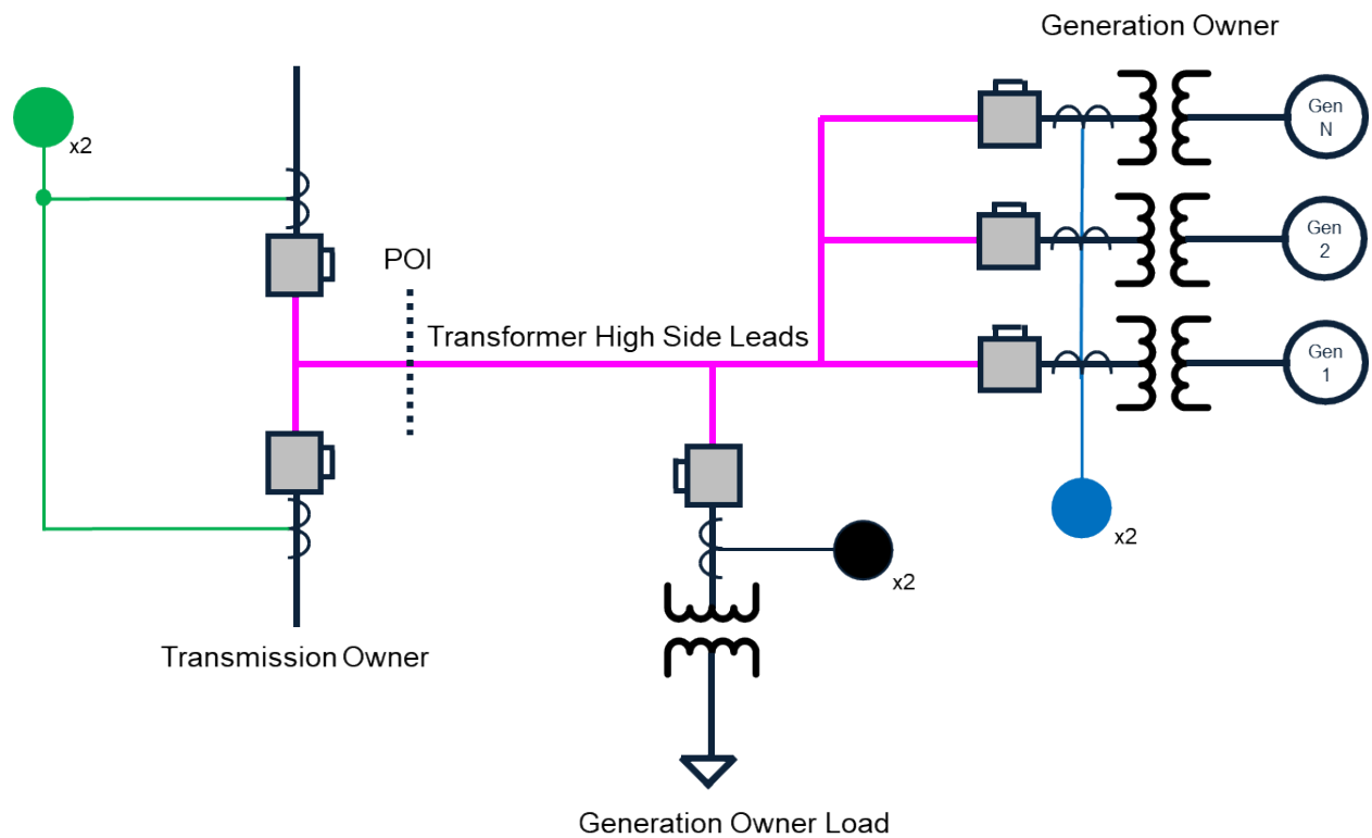
Figure 7. Prohibited Configuration
