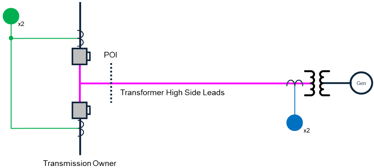
Figure 3. Acceptable Configuration
