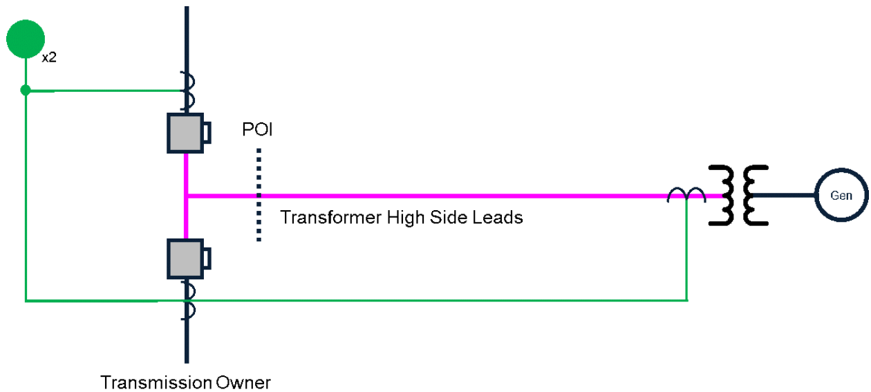
Figure 4. Acceptable Configuration
