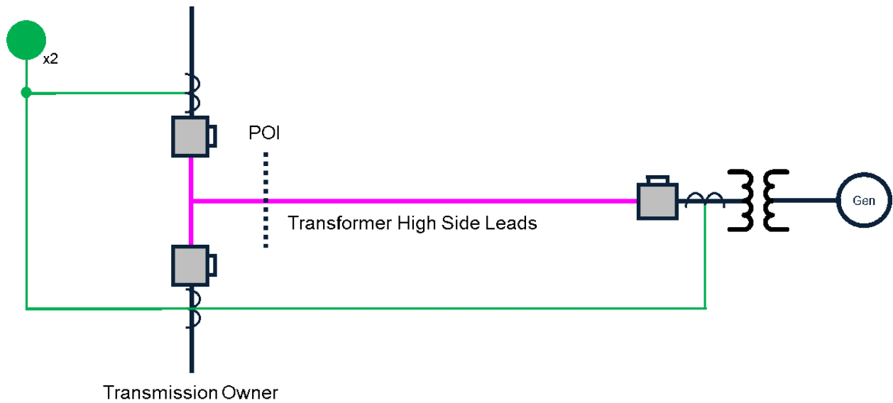
Figure 2. Acceptable Configuration
