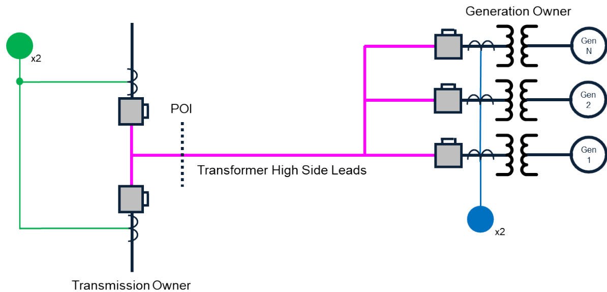
Figure 5. Acceptable Configuration
