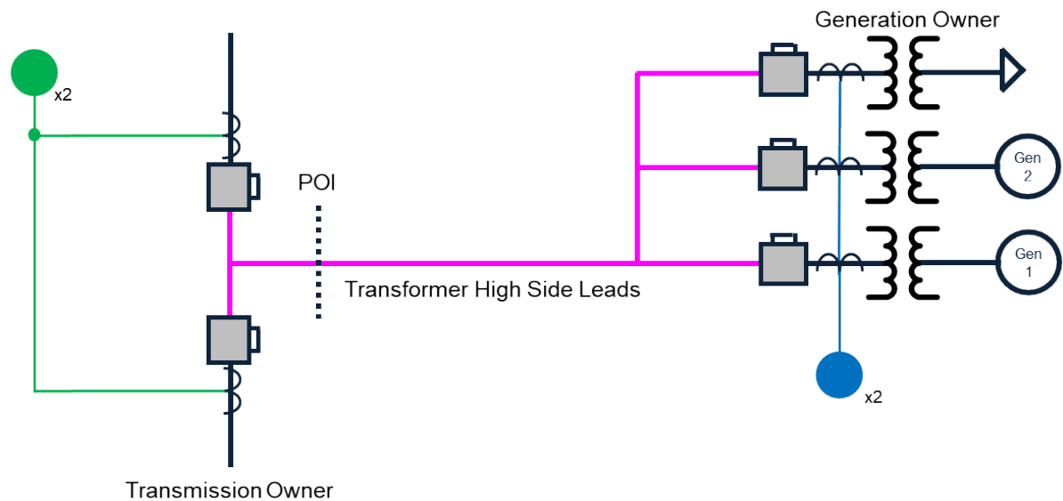
Figure 6. Acceptable Configuration
