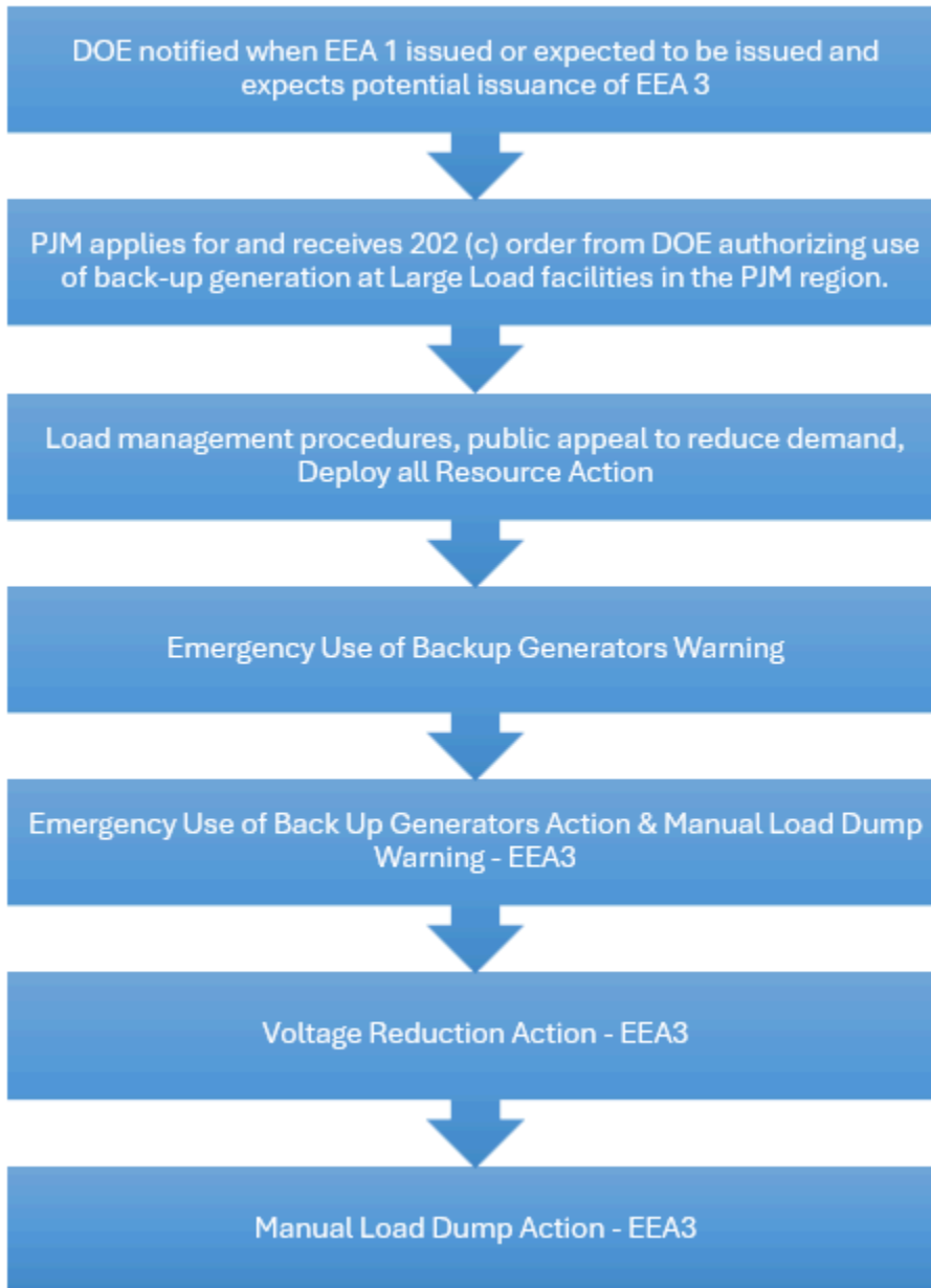
Exhibit 12: Emergency Use of Back-up Generators Process Flowpath Example
