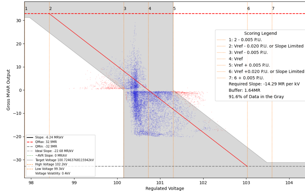
Gross MR Output vs. Regulated Voltage. 2026-02-02 07:40:00-05:00 through 2026-05-01 20:15:00-04:00
