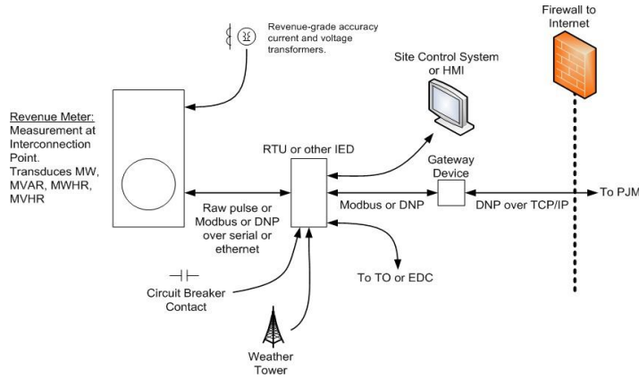
Exhibit 4: Typical Internet DNP Configuration
