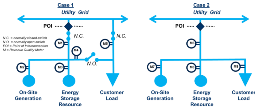
Exhibit 8: Energy Storage Resource Metering Example
