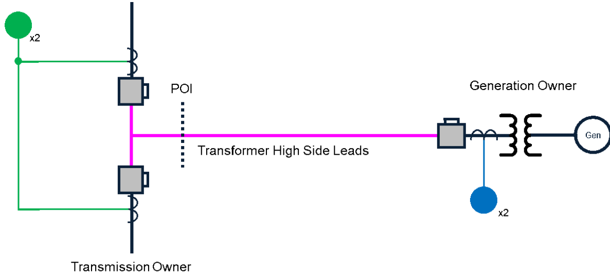
Figure 1. Acceptable Configuration
