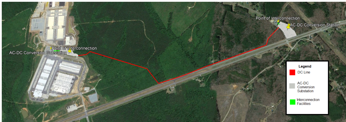
Exhibit 51: Merchant Transmission Request Site Plan
