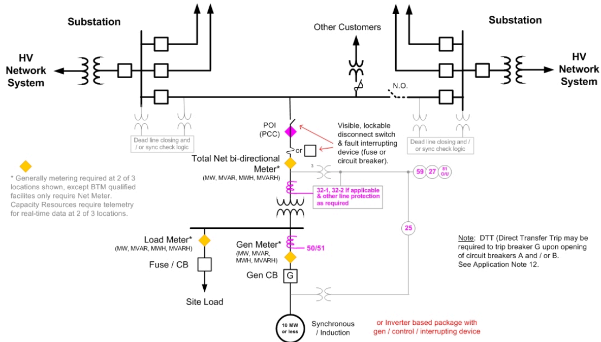
Figure 6C – One-Line Diagram for a Typical Interconnection to a Radial Transmission System
