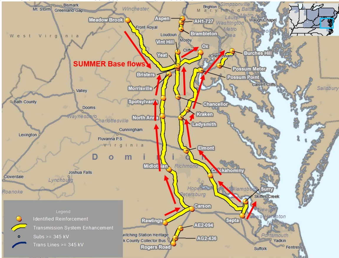
Map 4. 2025 RTEP Window 1: 2032 500 kV Dominion Violations
