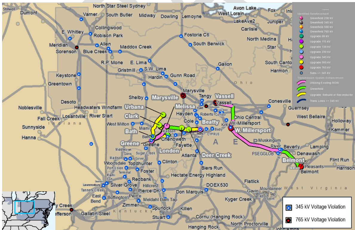
Map 34. Proposal 239: 2032 N-1-1 765 kV and 345 kV Voltage Violations
