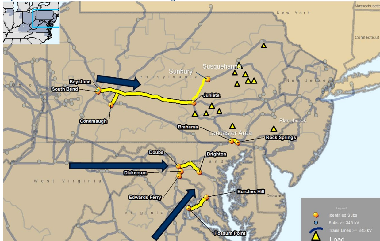
Map 5. 2032 Overloads in the PJM Mid-Atlantic Regions
