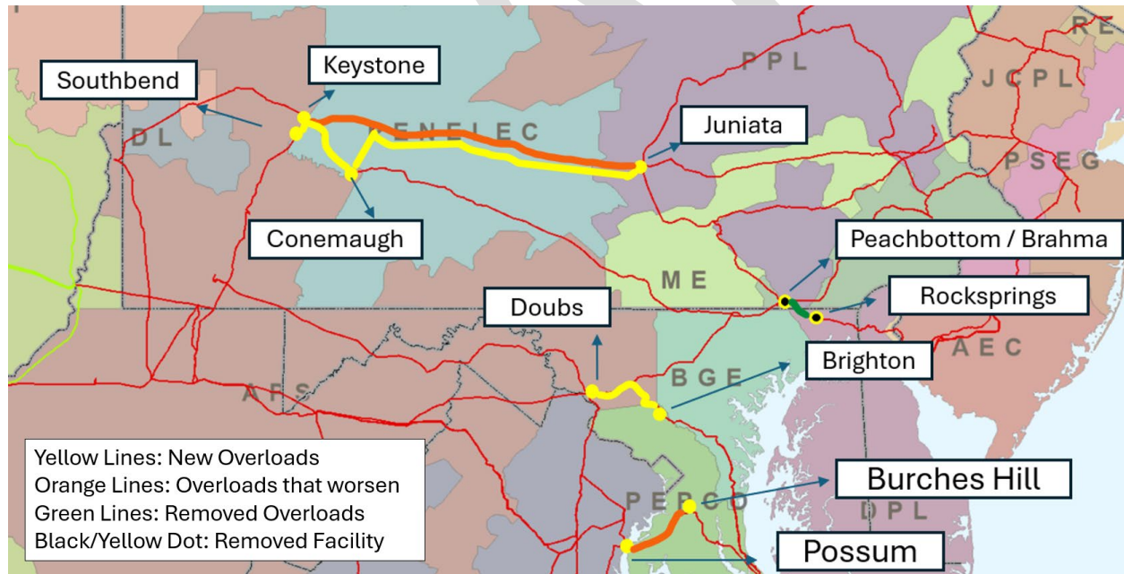
Map 1. 2025 RTEP Window 1: 2032 Scenario 4 MAAC Region 500 kV Violations
