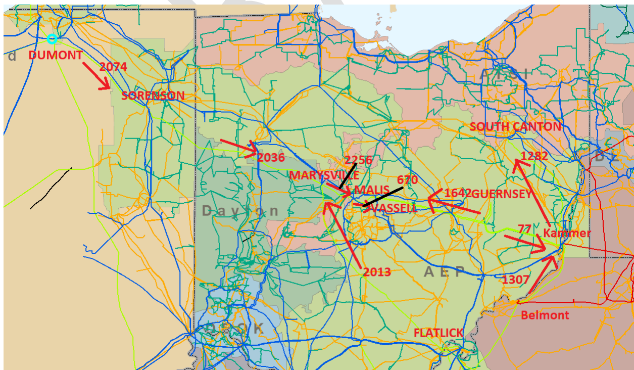
Map 14. 2030 Summer Base Case Flows on 765 kV Transmission Lines
