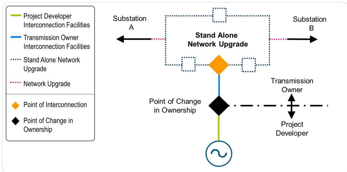
Exhibit 9: Generator Interconnection via New Interconnection Switchyard
