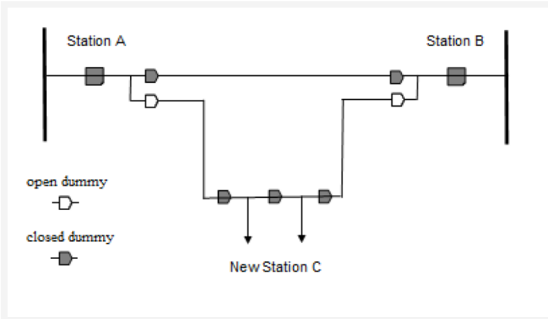
Exhibit 9: Dummy Switches to model new facilities pre- and post-construction
