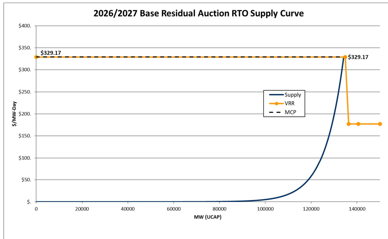
Figure 1. RTO Smoothed Supply (2026/2027 Base Residual Auction RTP Supply Curve)
