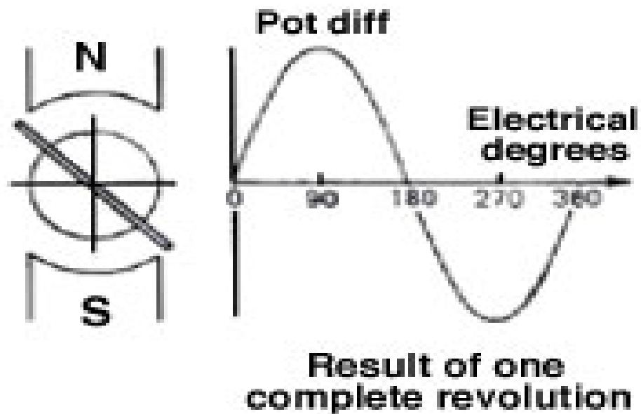
Two-pole generator
