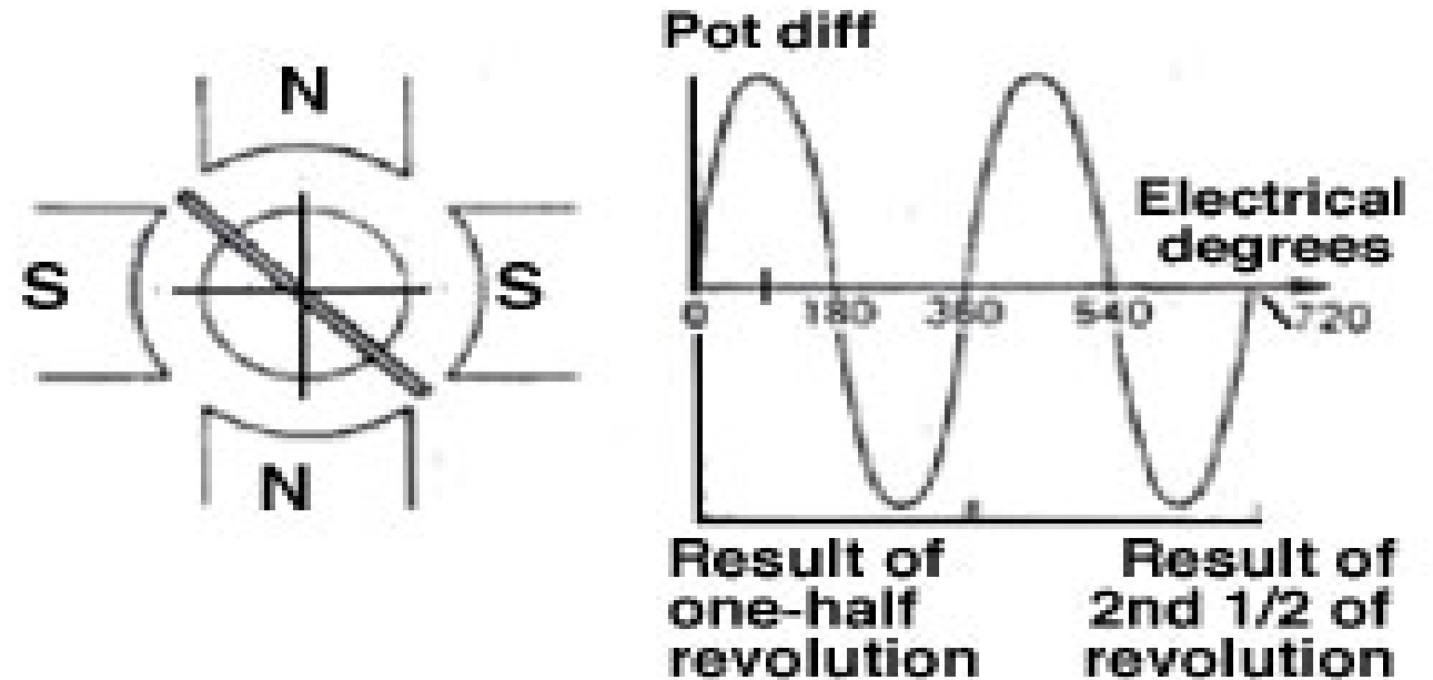
Four-pole generator
