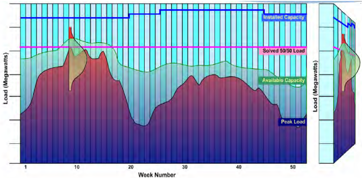
Exhibit 7: Daily load distribution
