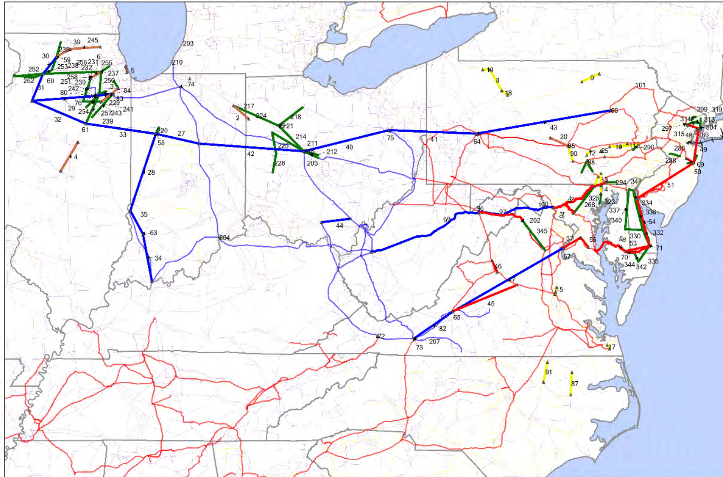
Map 4.3: EIPC Scenario 2 Transmission Overlay
