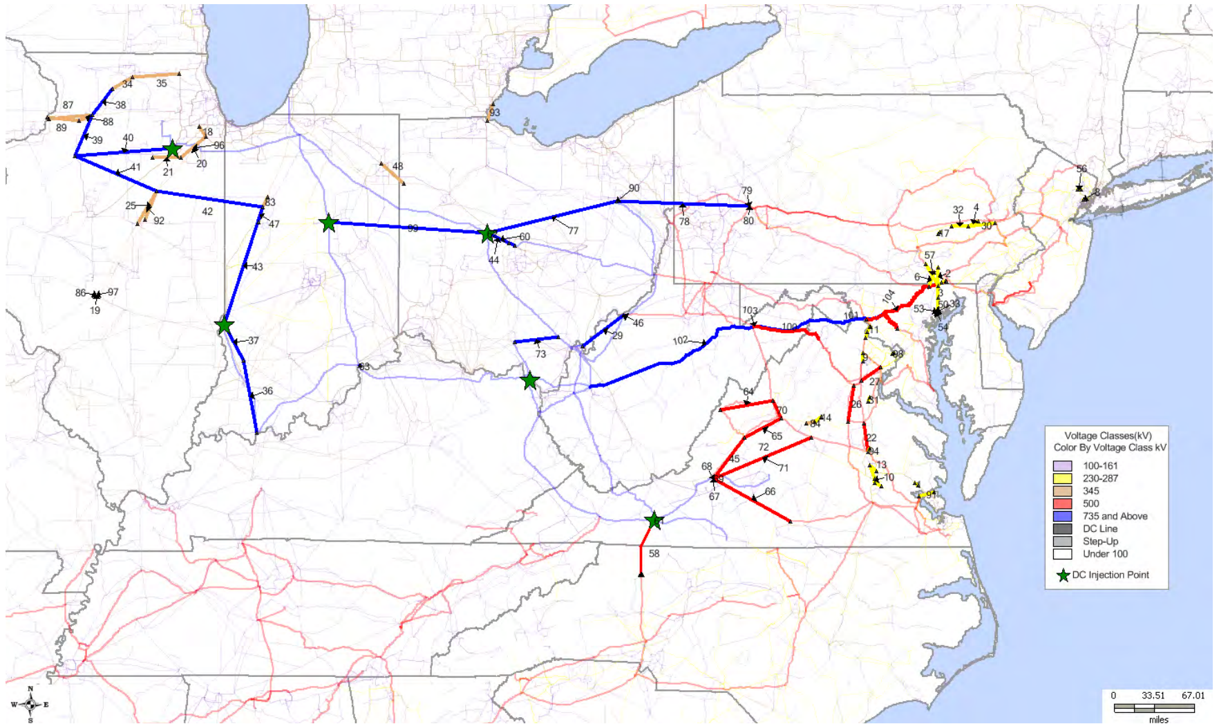
Map 4.2: EIPC Scenario 1 Transmission Overlay
