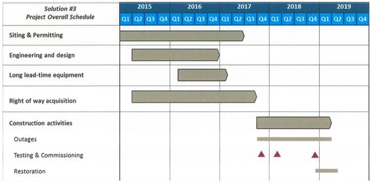
Figure C.4.1-1: Montour to Sunbury 230kV Single Circuit Integrated Schedule
