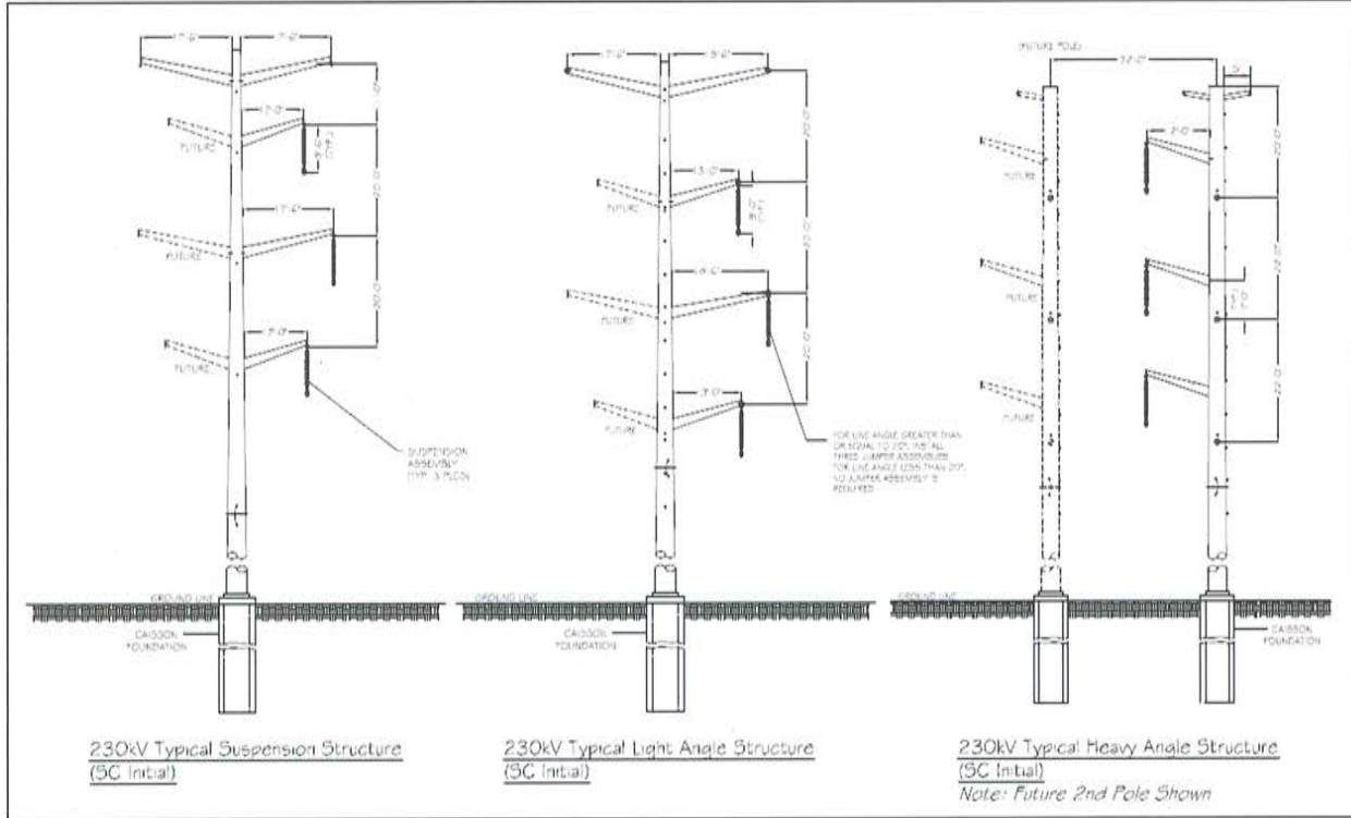
Figure C1.3-1: Typical 230kV Structure Types
