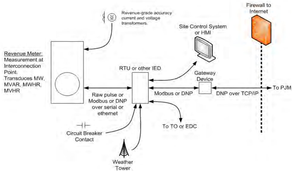
Exhibit 5: Typical Internet DNP Configuration
