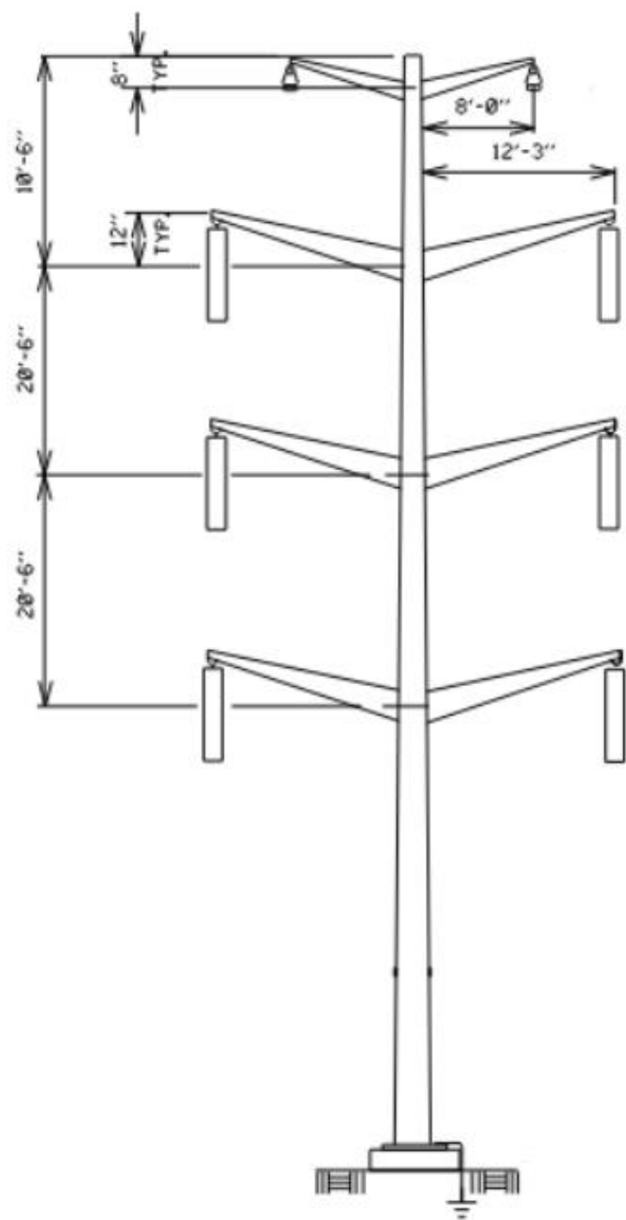
Figure 2 – Proposed Suspension Structure Configuration
