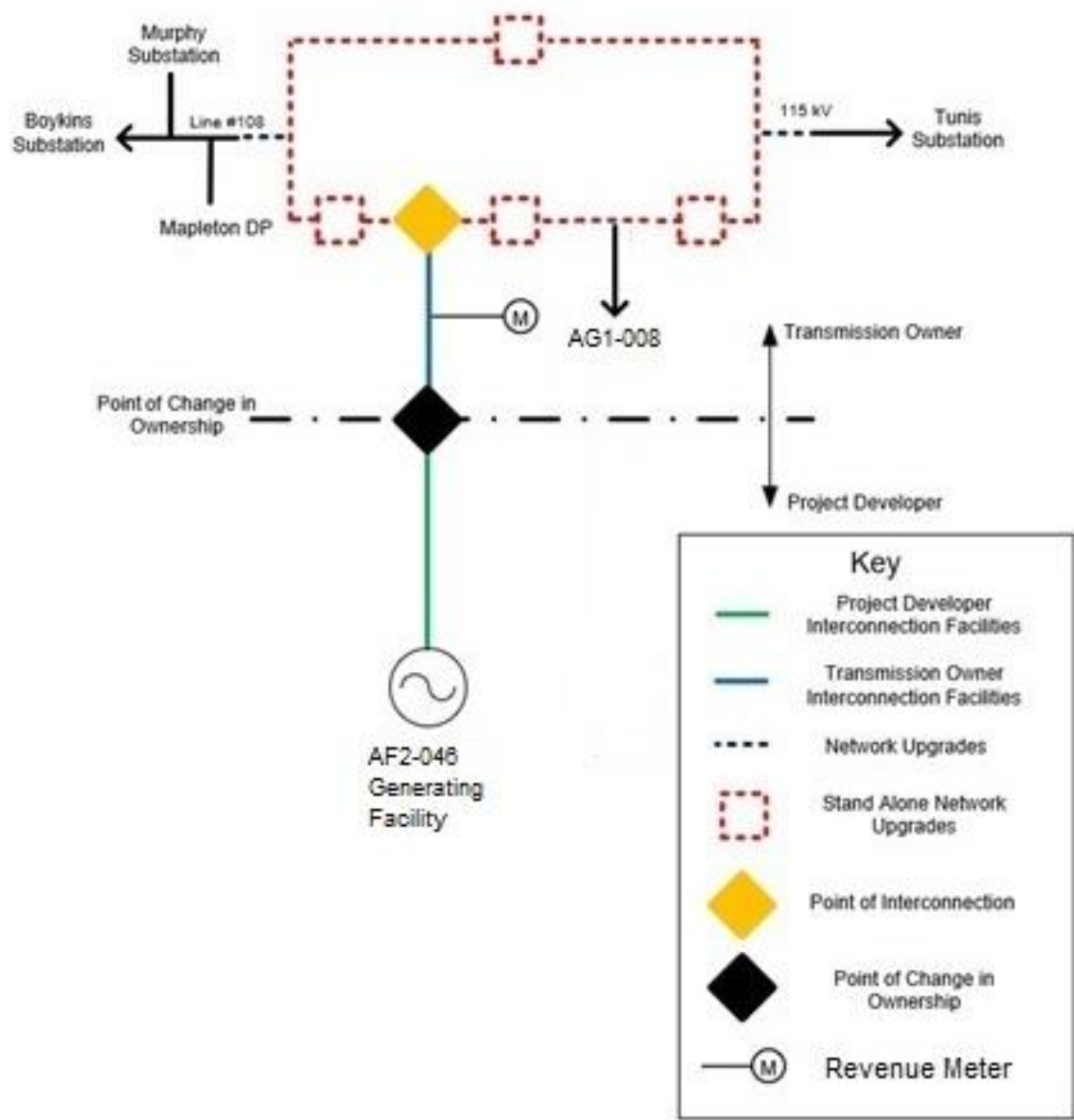
Attachment #1: Single line Diagram for the Physical Interconnection
