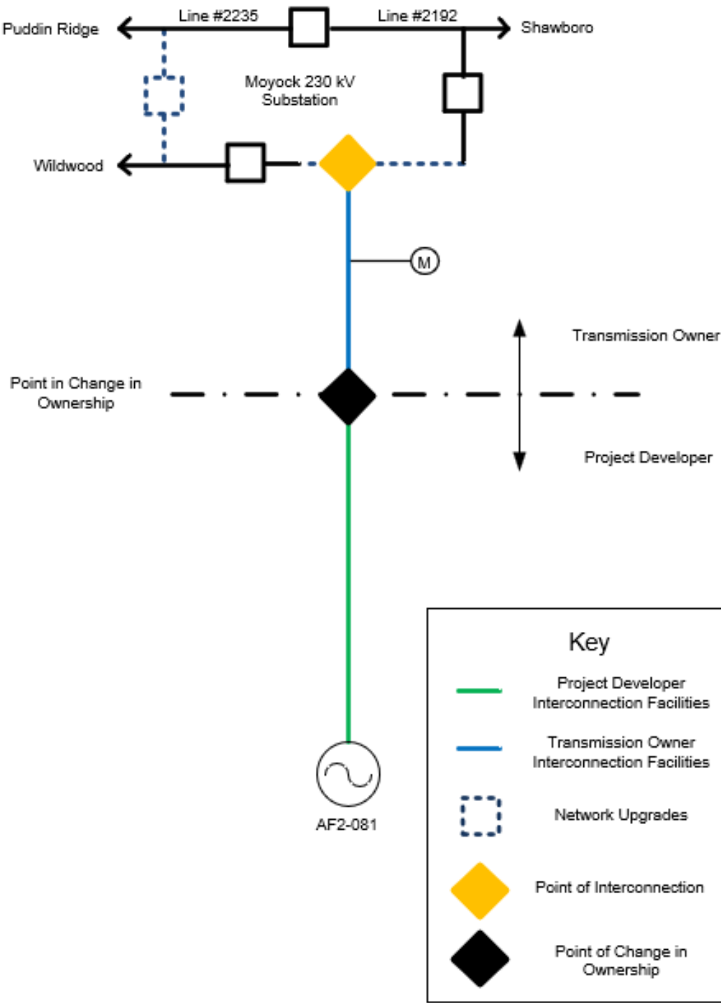
Attachment #1: Single line Diagram for the Physical Interconnection
