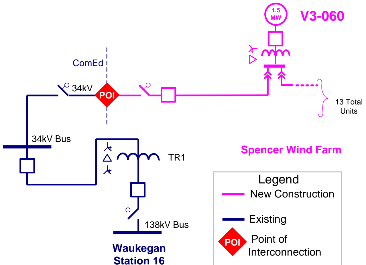
Figure 1. Proposed Interconnection Single Line Diagram
