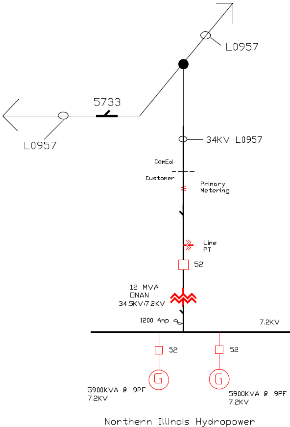
Figure 1. Proposed Interconnection Single Line Diagram
