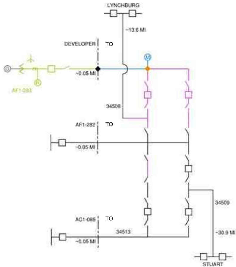
AF1-283 CLAY SUBSTATION 345 KV
