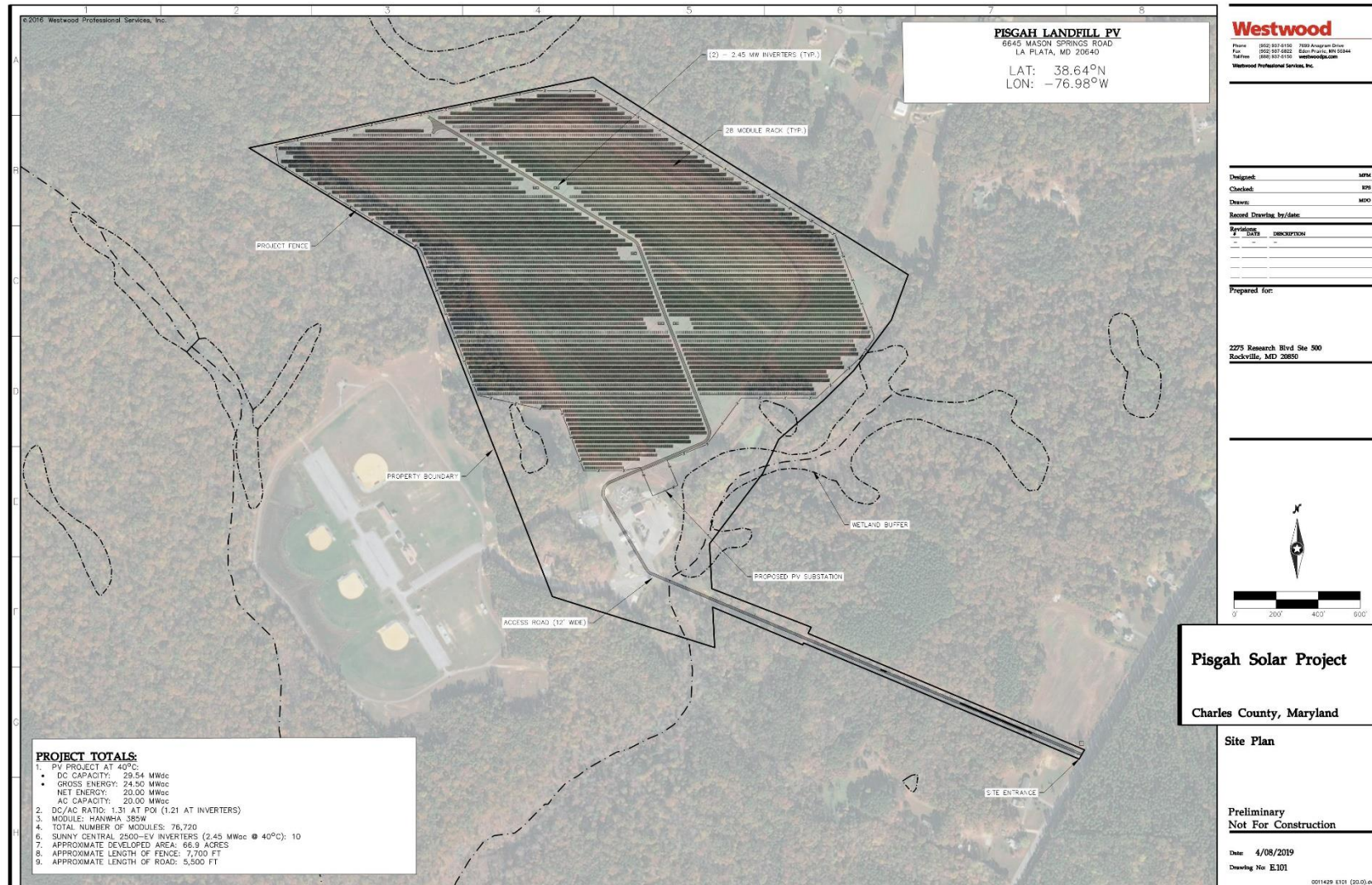
Figure Two – Proposed Solar Developer Site Plan and Location
