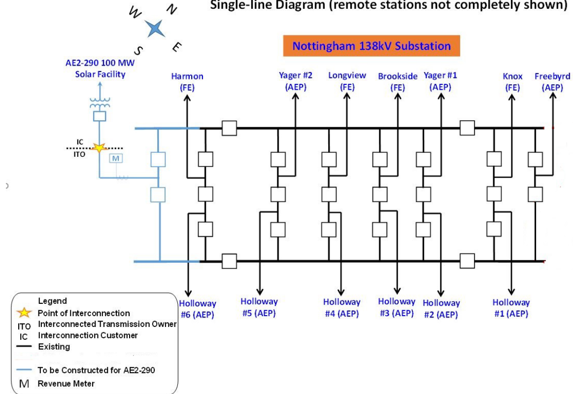
AE2-290 Point of Interconnection Nottingham 138 kV Single-line Diagram (remote stations not completely shown)
