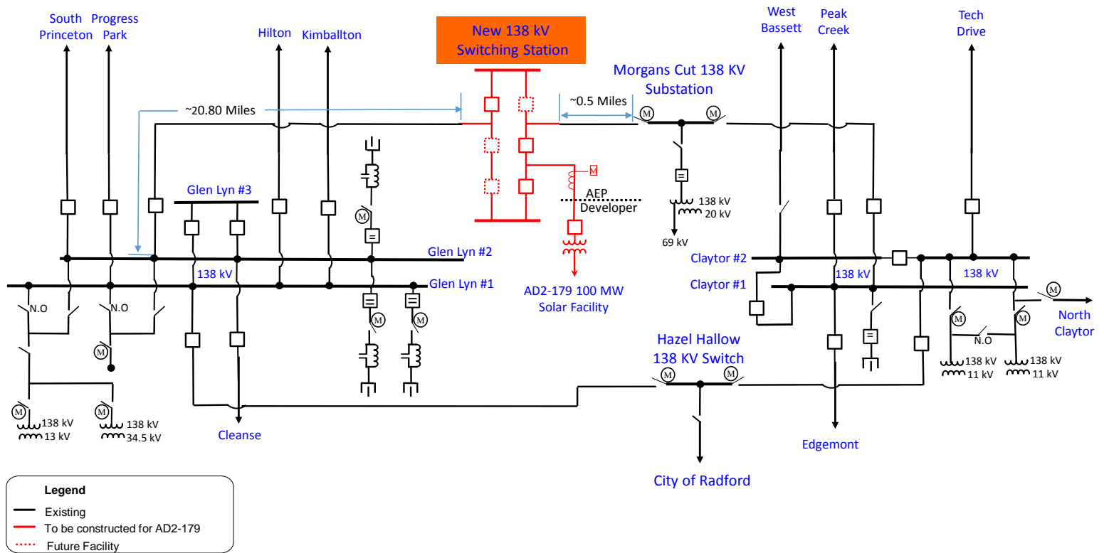
AD2-179 Primary Point of Interconnection (Morgans Cut – Glen Lyn 138 kV)
