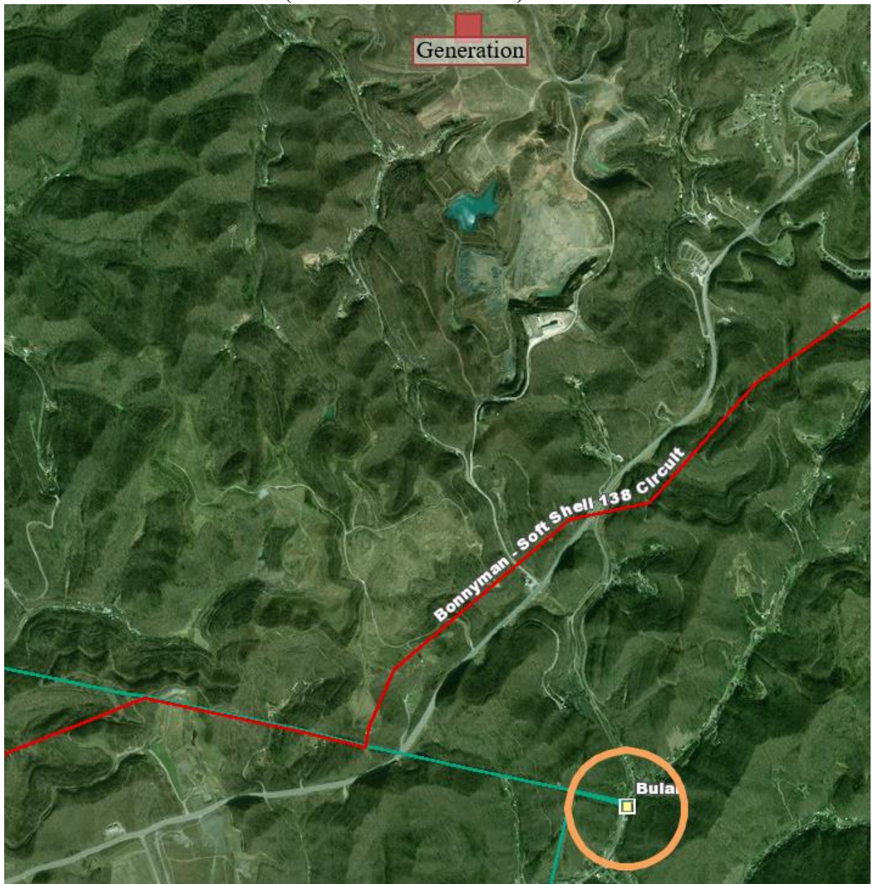
Figure 2: Customer Project Site and Primary Point of Interconnection (Bulan 69 kV Substation)
