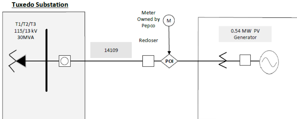
Figure 1 Single Line Interconnection Diagram
