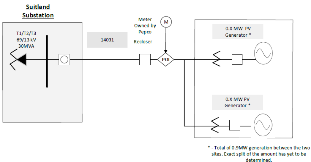
Figure 1 Single Line Interconnection Diagram
