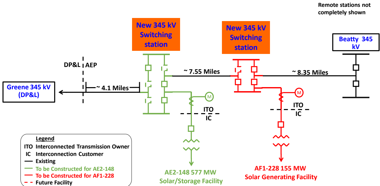
AF1-228 Point of Interconnection Beatty (AEP)– Greene (Dayton) 345 kV Circuit Single-line Diagram
