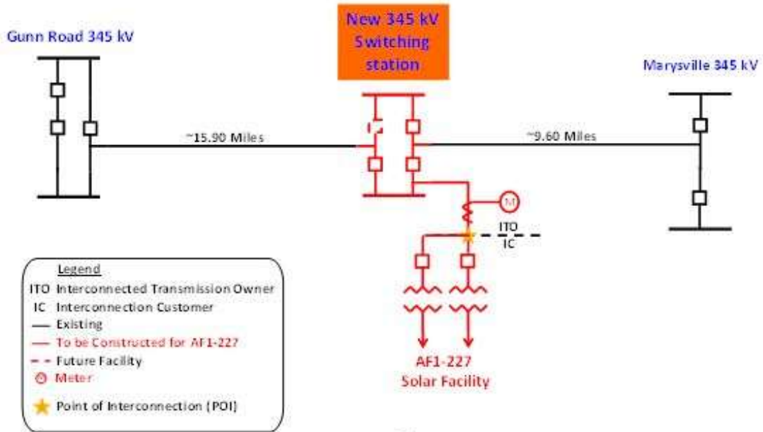
AF1-227 Point of Interconnection Marysville – Gunn Road 345 kV Circuit Single-line Diagram
